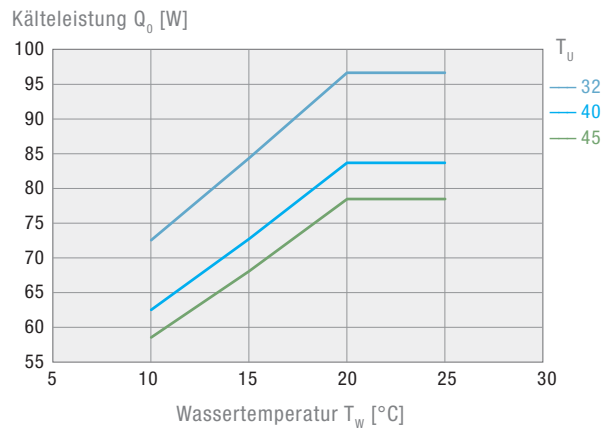
EB XT 1000 WT (50 Hz) 1
