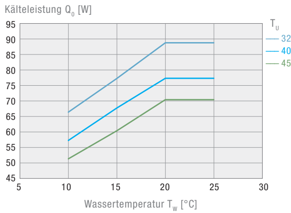
EB XT 900 WT (50 Hz) 1
